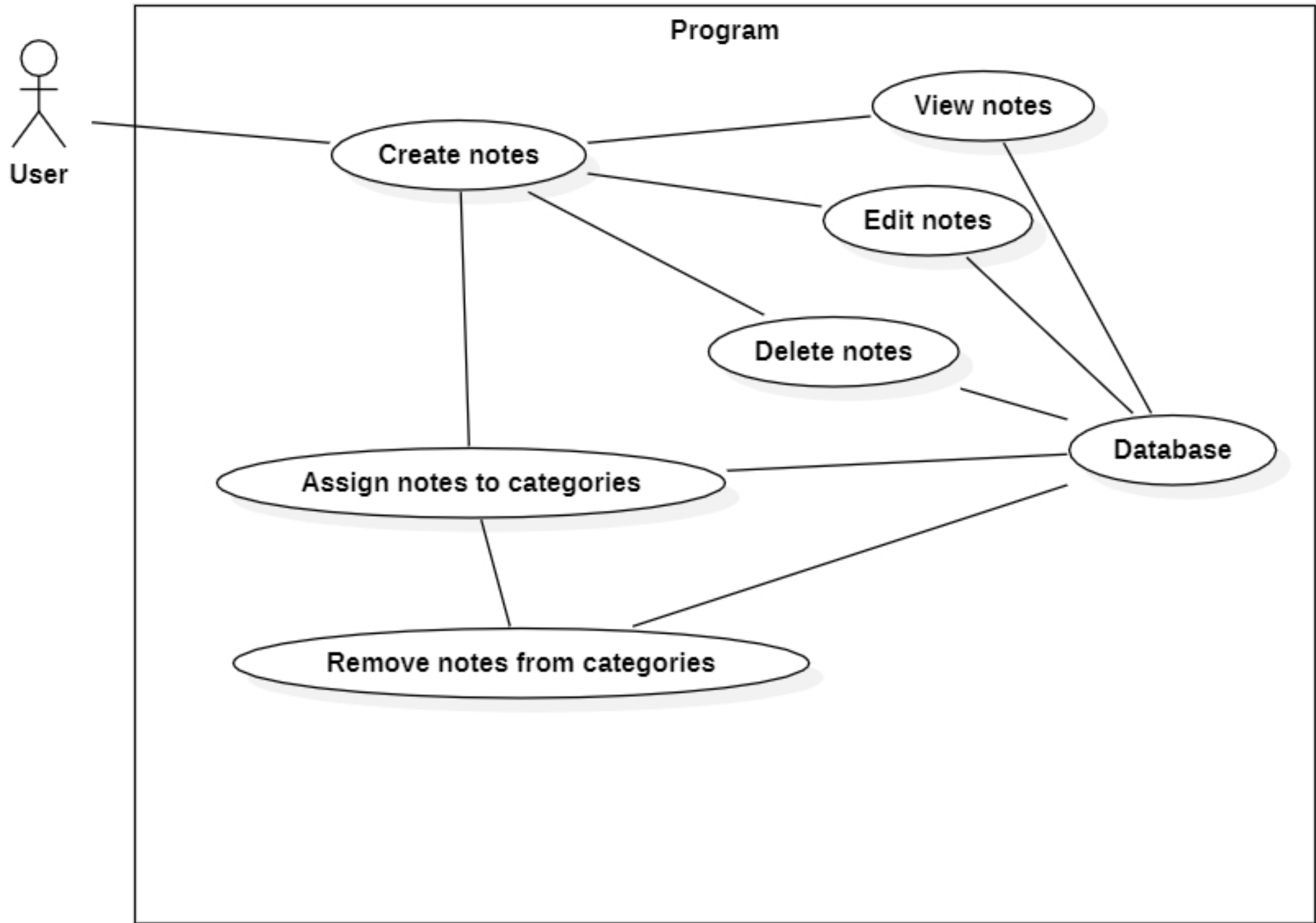
Use case diagram for note taking application
